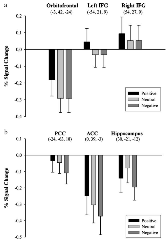
Fig. 4. Percent signal change and associated standard errors for positive, neutral and negative words at the peak of the hemodynamic response at regions indicated (IFG inferior frontal gyrus, ACC anterior cingulate gyrus, PCC posterior cingulate gyrus).
