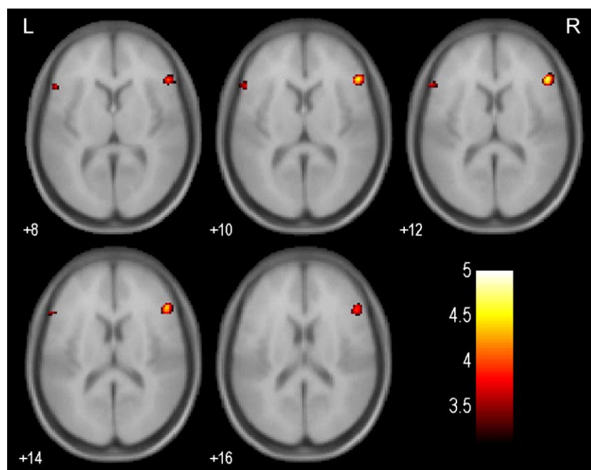
Fig. 2. Inferior frontal gyrus activity identified in the valence independent emotional > neutral contrast displayed on MNI 305 brain average ( P < 0.001, uncorrected). The numbers at the left bottom corner indicate z coordinate in MNI space. The color bar indicates the T values. L = left, R = right.
