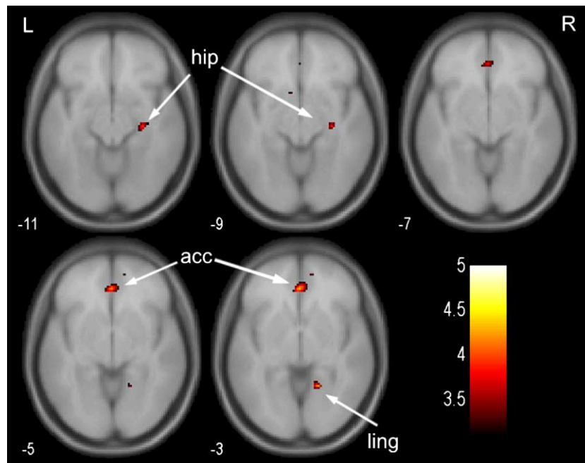
Fig. 3. Hippocampus (hip), anterior cingulate gyrus (acc) and lingual gyrus activity (ling) as identified in the positive > negative contrast ( P < 0.001 , uncorrected).
