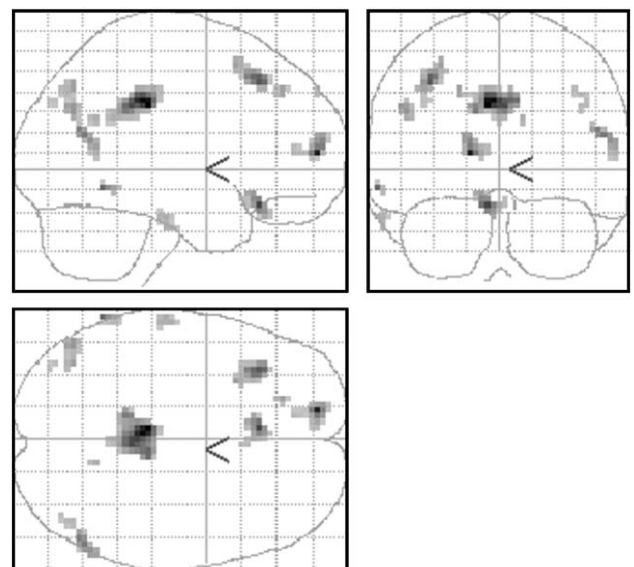
Fig. 1. Maximum intensity projections illustrating voxels common to word > nonword contrast (thresholded at P < 0.001 , uncorrected).
